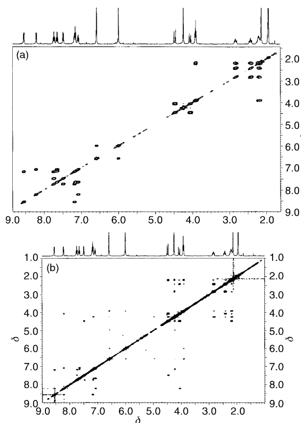
Fig. 2 1 H NMR spectra of complex 2 in d 3 -acetonitrile solution recorded on a Bruker 400 MHz instrument at 298 K. (a) COSY, (b) NOESY.
